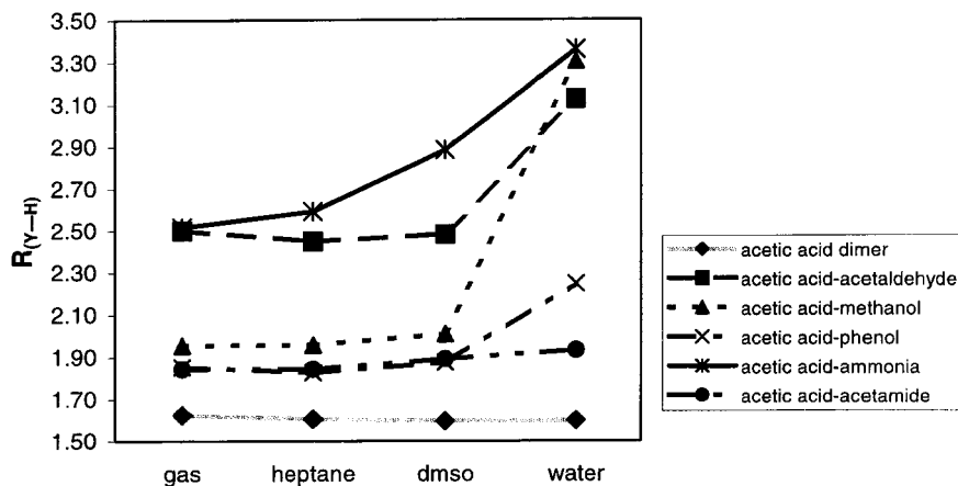
Figure 5. Hydrogen bond distances Y\cdots H (Å) of the weaker hydrogen bond for neutral complexes in gas and liquid phases.
