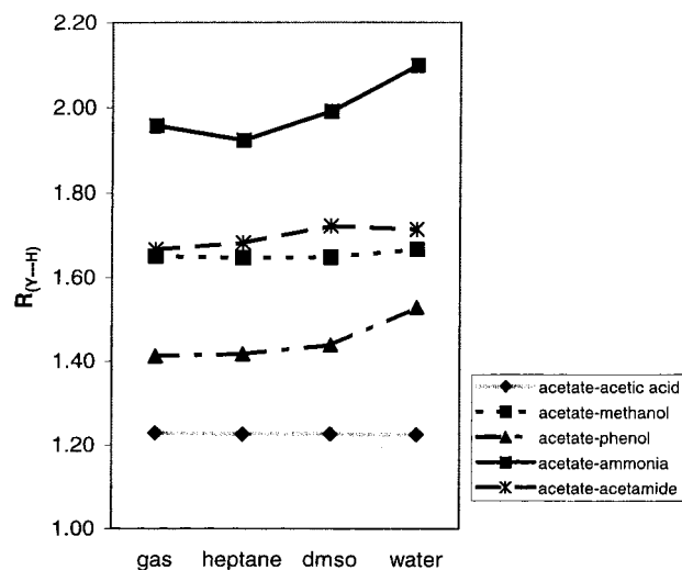
Figure 7. Hydrogen bond distances Y...H (Å) of the charged complexes in gas and liquid phases.
